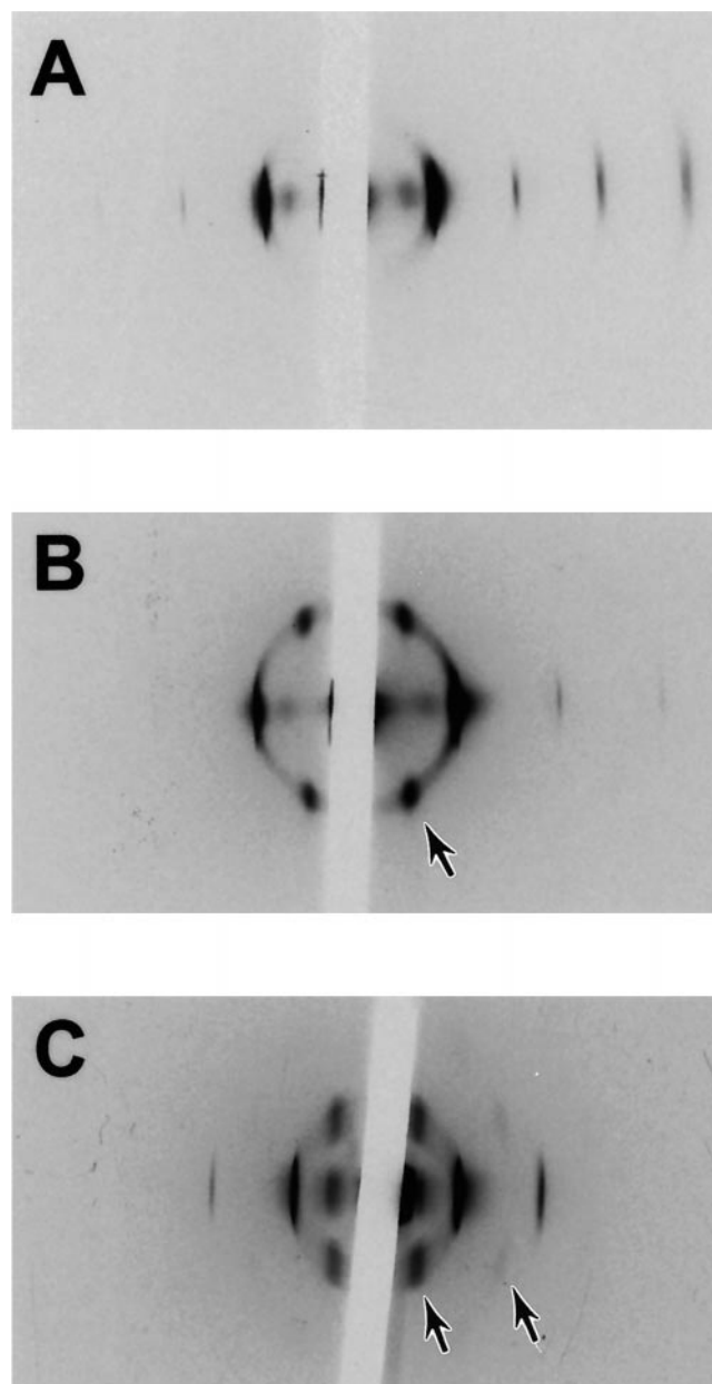
FIGURE 6 X-ray diffraction patterns for ( A ) EPC containing 10 mol% GMO at 98% relative humidity ( \log P = 7.5 ), ( B ) EPC containing 10 mol% GMO at 32% relative humidity ( \log P = 9.2 ), and ( C ) EPC containing 30 mol% GMO at 98% relative humidity. The x-ray patterns were recorded from lipid dried on a glass support oriented horizontally. The shadow of the rectangular beam stop is near the center of each pattern. The reflections on the left-hand side of each pattern are lighter than those on the right-hand side because of absorption of x-rays by the glass support. A is a typical pattern from oriented bilayers, showing equally spaced lamellar reflections on the equator of the film, oriented perpendicular to the planar bilayers. Patterns B and C display dark, sharp spots located off the equator of the film that fall on a hexagonal lattice. In B the arrow points to the (11) reflection, and in C the arrows point to the (11) and (21) reflections.
